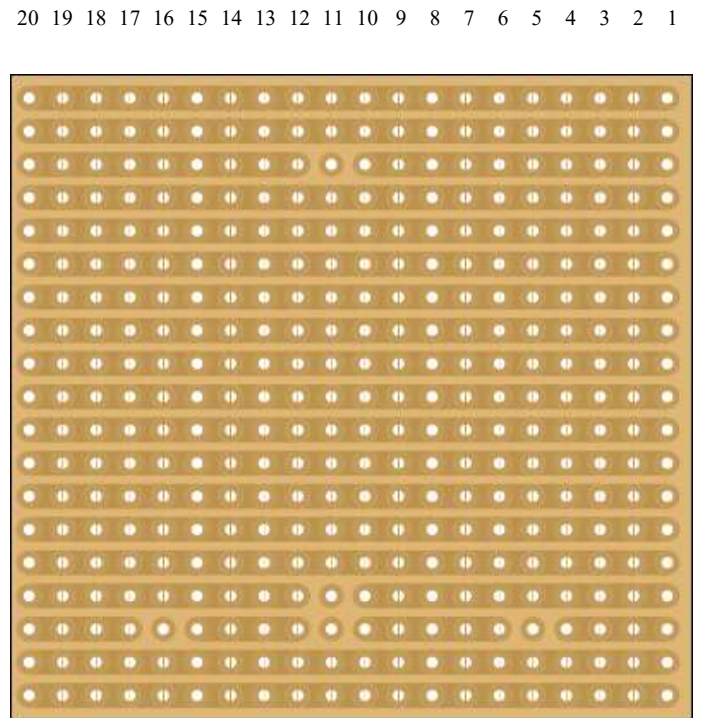
Copper Strip Side with Trace Breaks
